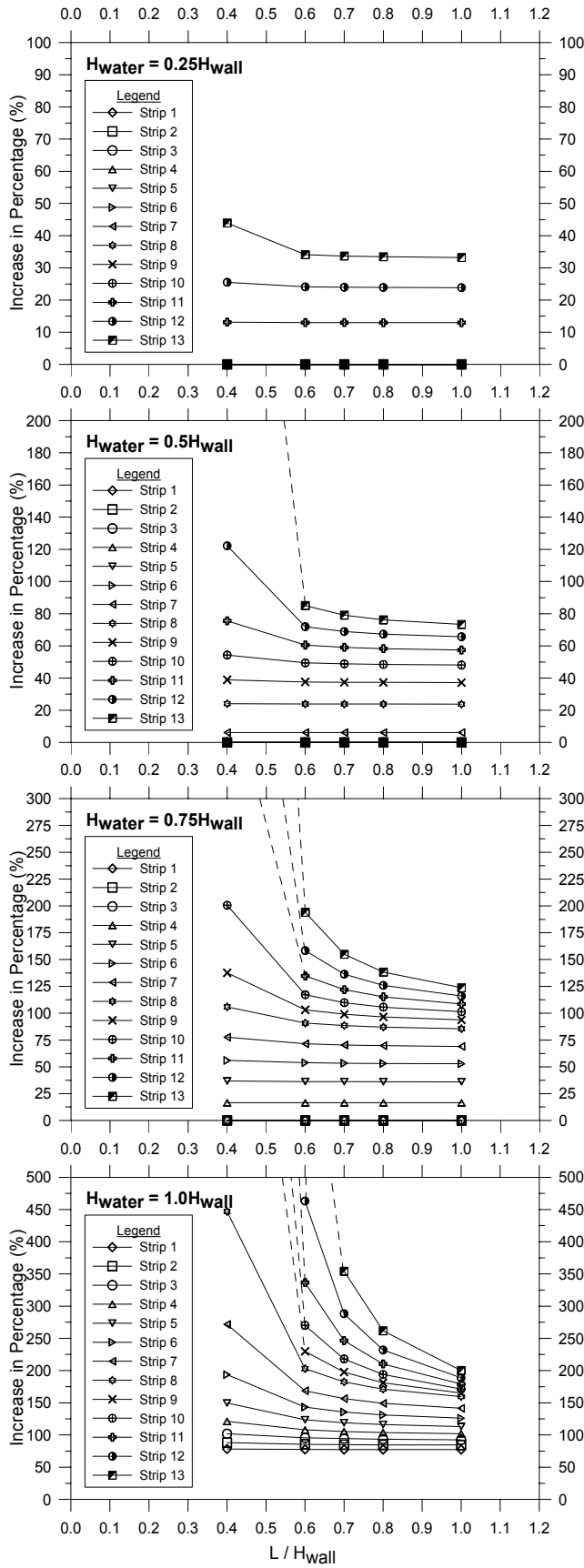
Fig. 6 Variation of maximum acting tensile force for each layer of reinforcement.
