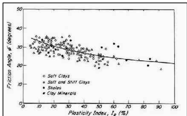
Figure 22 : Values of \phi' for Clays of Various Compositions as Reflected in Plasticity Index (from Terzaghi et. al.,1996)
