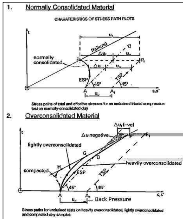
Figure 21 : Stress Path for CIU Tests on NC & OC Soils
