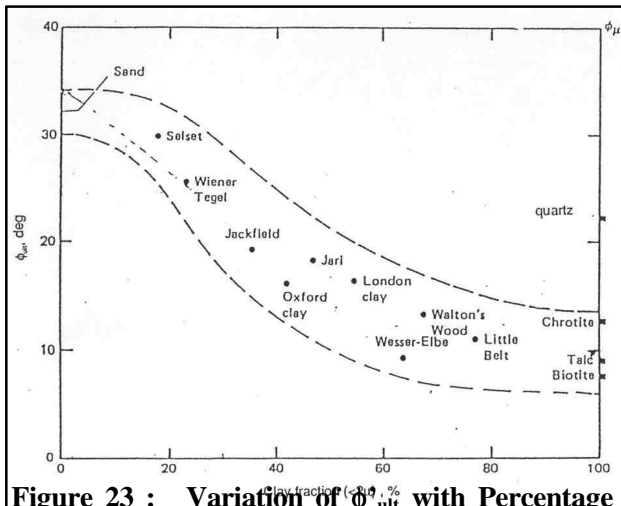
Figure 23 : Variation of \phi_{ult} with Percentage of Clay Content (after Skempton, 1964)
