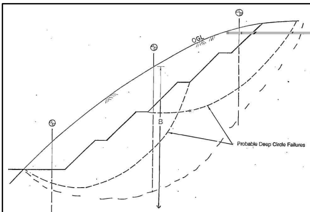
Figure 1 : Depth of Field Tests for Stability Analysis
