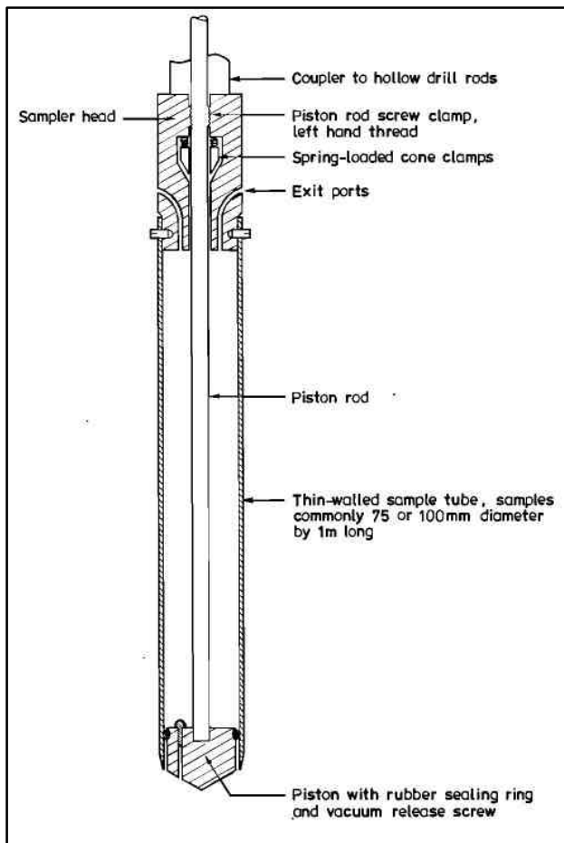
Figure 6 : Piston Sampler
