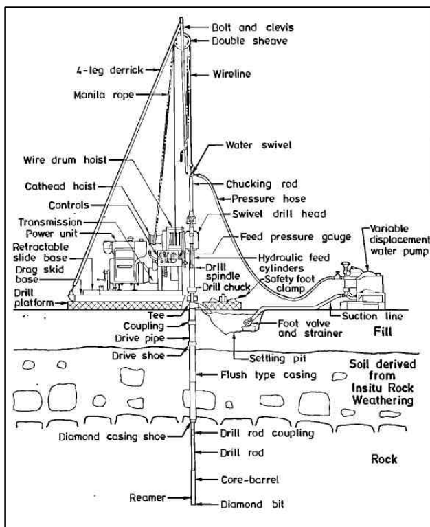
Figure 4 : Typical Rotary Drilling Rig (from Geoguide 2, 1987)
