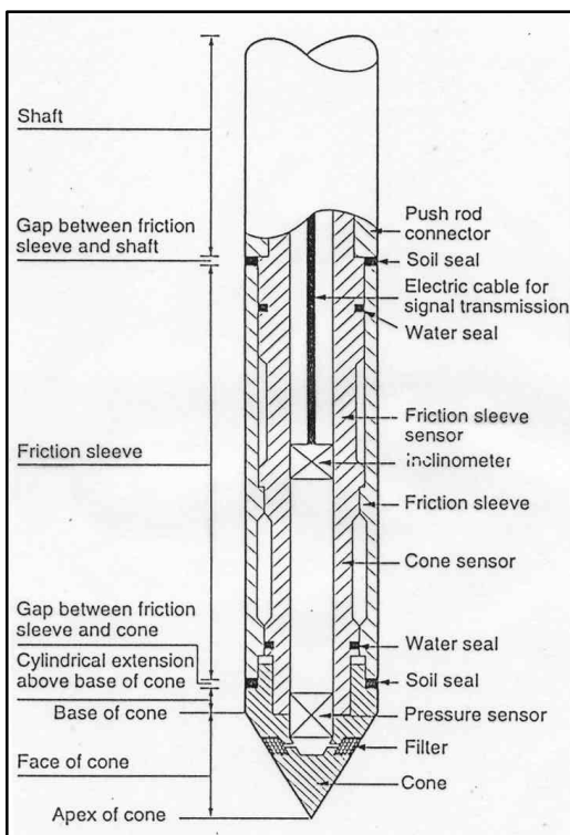
Figure 10 : Detailed Terminology of Piezocone
