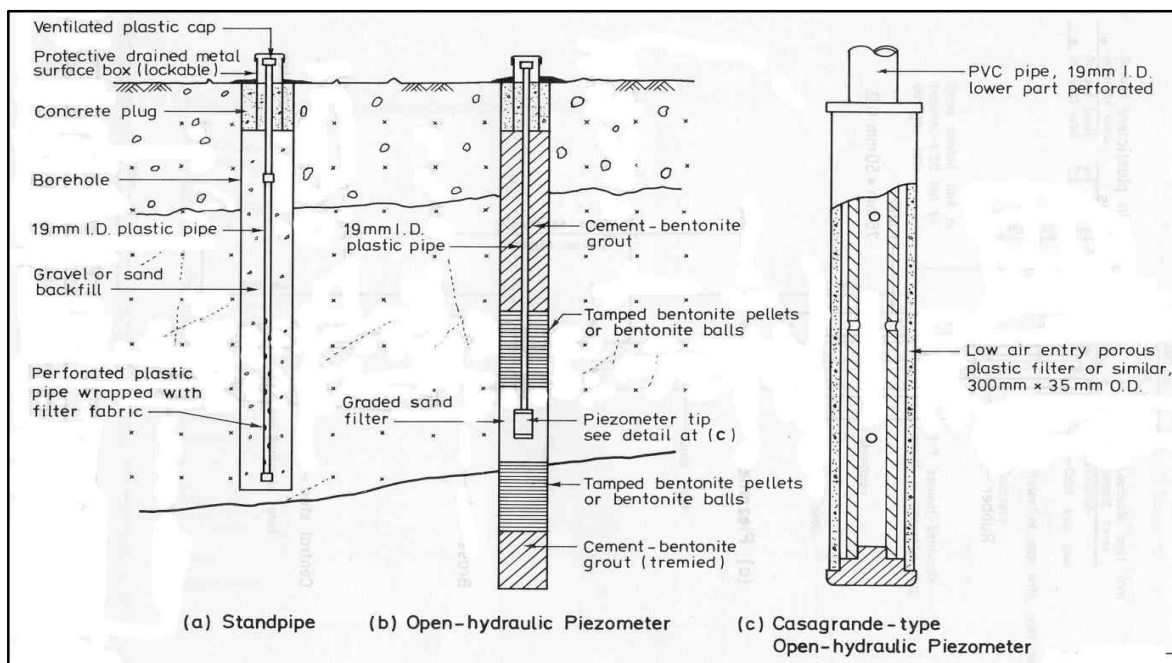
Figure 13 : Typical Standpipe and Open-Hydraulic Piezometers (after Geoguide 2, 1987)
