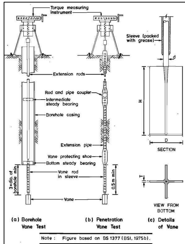
Figure 9 : Field Vane Shear Devices
