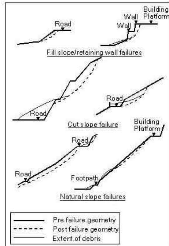
Figure 4 : Typical Slope Failures in Residual Soils (modified from GCO, 1991)
