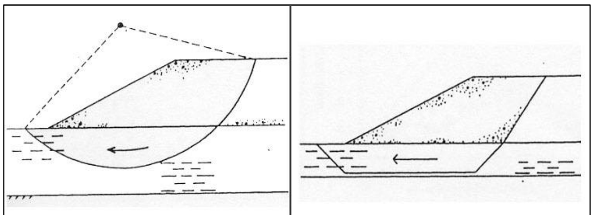
Figure 2 : Circular & Non-Circular Failure Surfaces
