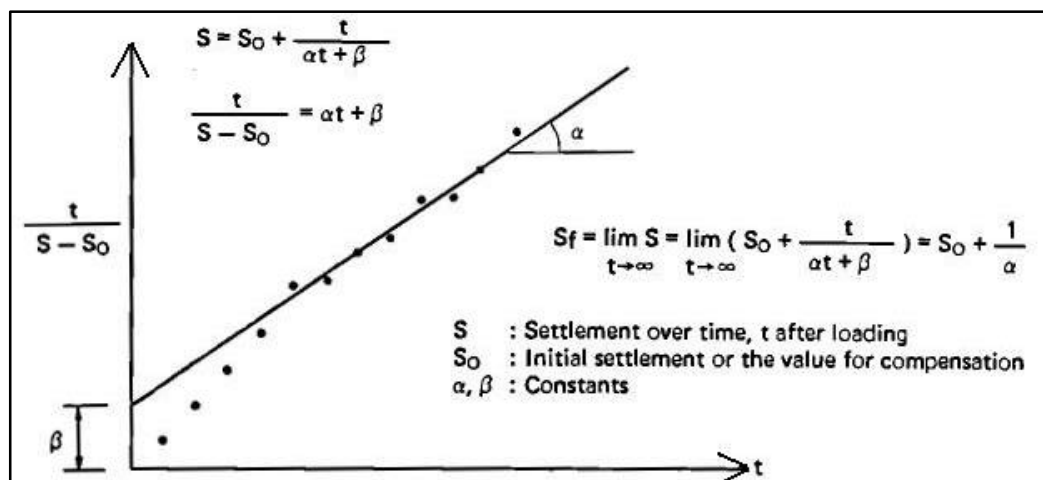
Figure 13 : Hyperbolic Method to Predict Future Settlement
