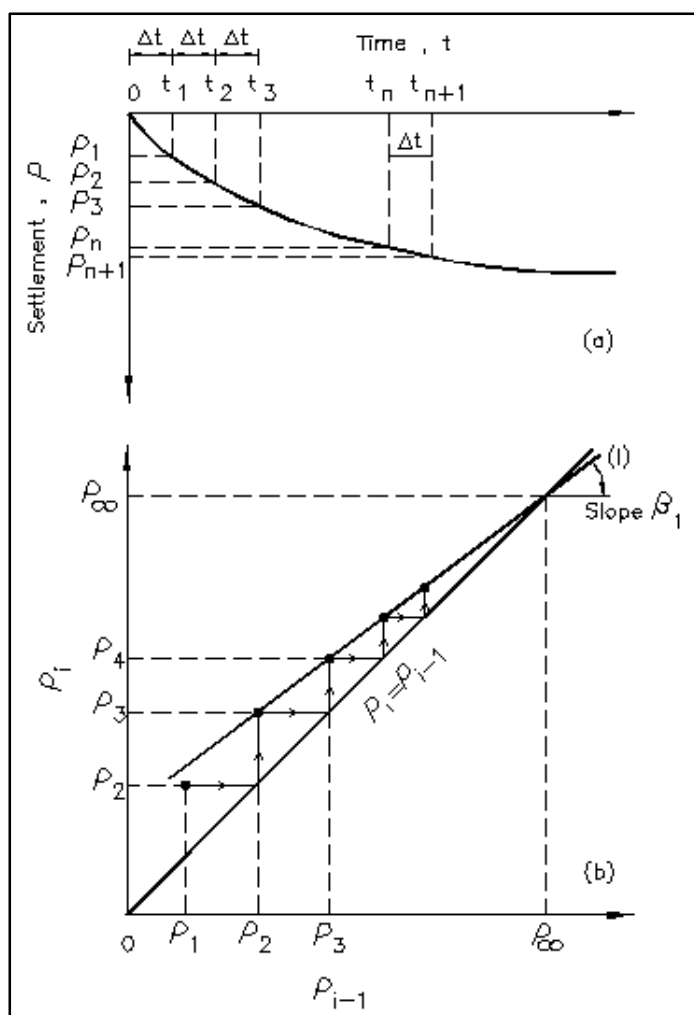
Figure 16 : Graphical Method of Asaoka
