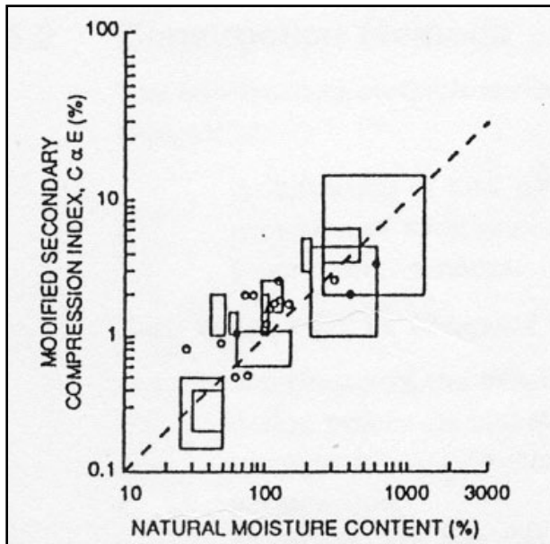
Figure 7 : Relation between Secondary Compression Ration and Water Content (from Mesri, 1973)
