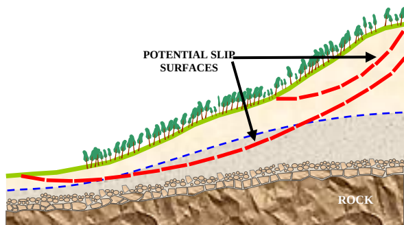
Figure 6: Potential Slip Surfaces
