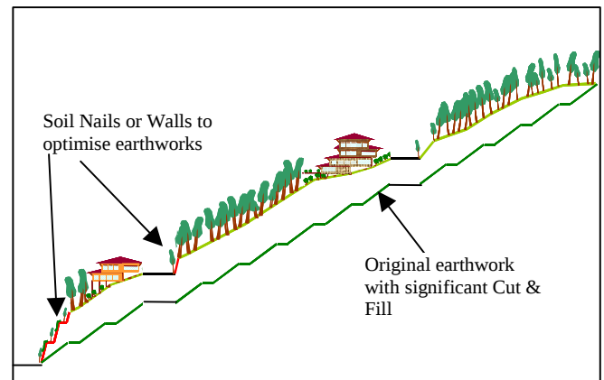
Figure 2 : Method to Optimise Earthworks
