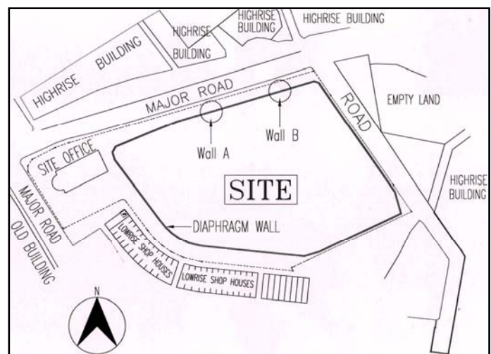
Figure 1. Site plan.
