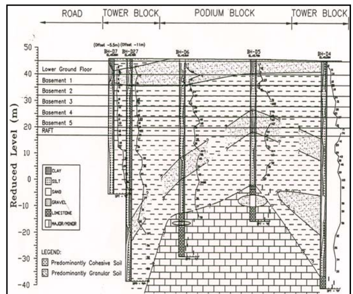
Figure 2. Typical subsoil profile (from Tan 1997).
