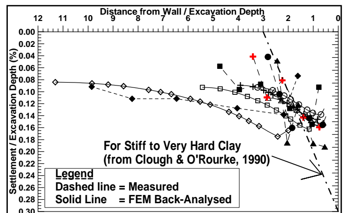
Figure 8. Dimensionless ground surface settlement profile.
