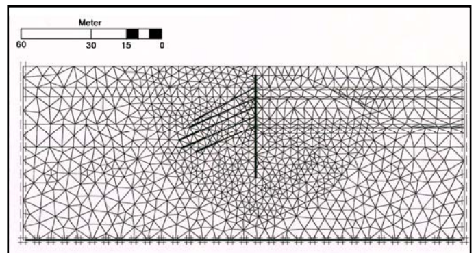
Figure 3. Finite element modelling of excavation.
