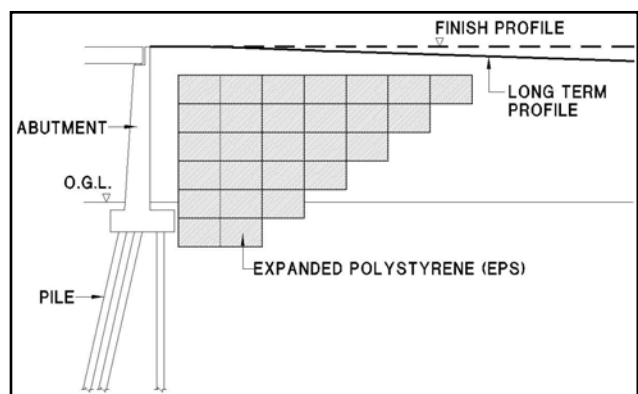
Figure 4 : Use of EPS at Bridge Abutment
