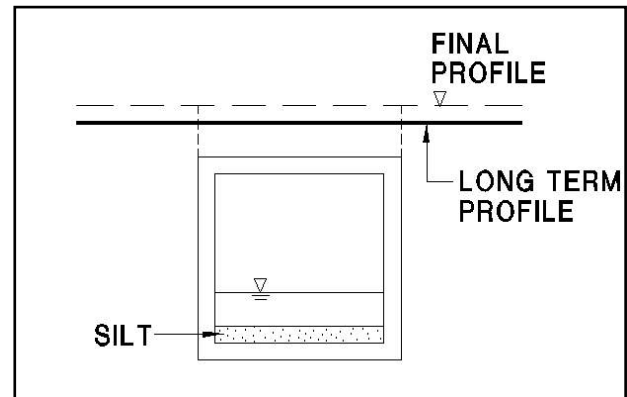
Figure 8 : Oversized Culvert
