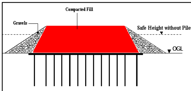
Figure 6 : Typical Piled Embankment Section
