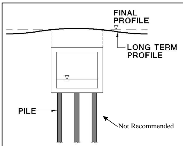
Figure 7 : Piled Culvert (Not Recommended)
